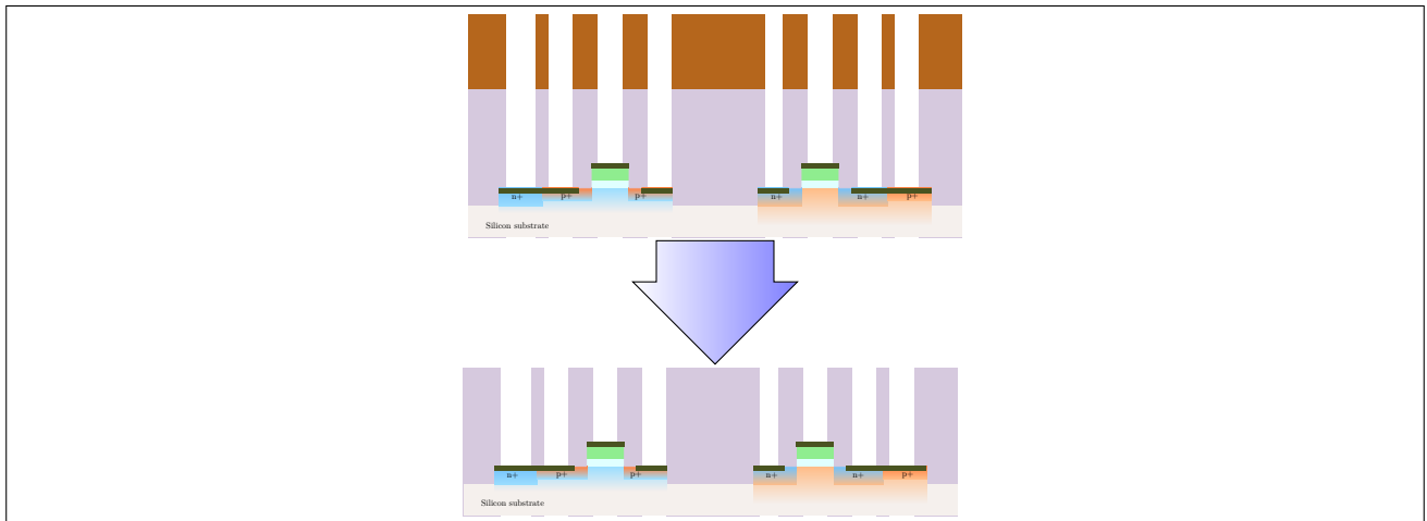
Figure 69: Resist removal
