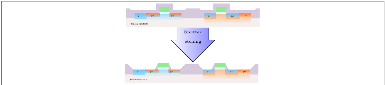
Figure 59: Anisotropic etching
