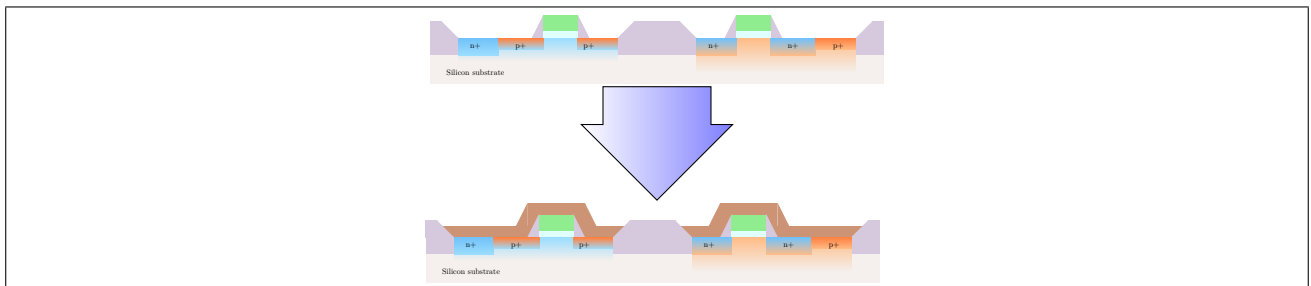
Figure 60: Titanium deposition
